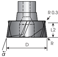
6 flutes D:16-25mm
