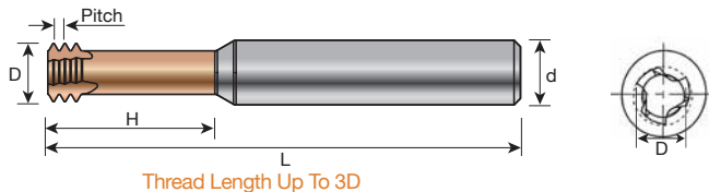
Thread Length Up To 3D
